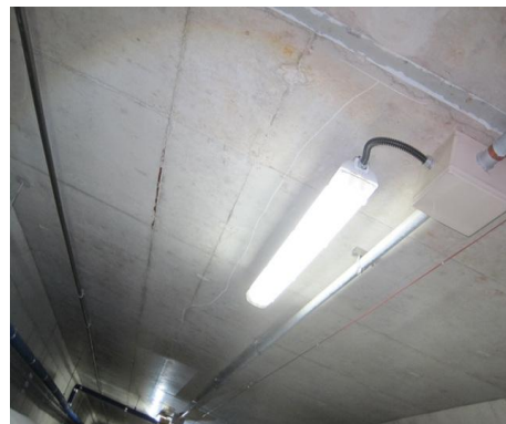
1련 Sta.0+87m 중균열(cw=0.1mm, L=4.0m)
